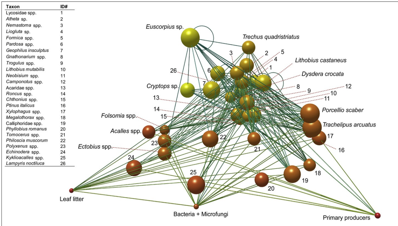
Figure 2.8 As one emblematic example of a food web from the brown world, we show here the soil and litter arthropod network of the Monte Venere beech forest (Lake Vico, Italy) plotted using Network3D . Representative taxa are directly reported, other taxa are coded (IDs 1–26) and shown in the upper legend. Node diameters of each taxon are proportional to the specific log-transformed body-mass average ( \mu\text{g} dry weight); the mass of primary producers, leaf litter and microbes are arbitrarily set to 10 \mu\text{g} to improve the graph readability. Node heights are proportional to the mean \delta^{15}\text{N} value of each taxon. The \delta^{15}\text{N} signature of leaf litter is set at -2.13 , corresponding to the signature of decaying Fagus sylvatica leaves sampled in the upper soil layer. An identical signature was assumed for all basal resources (i.e. primary producers, bacteria and fungi) for demonstrative purposes. The vegetation of the entire study area has been described in Scoppola et al. (1989) .
