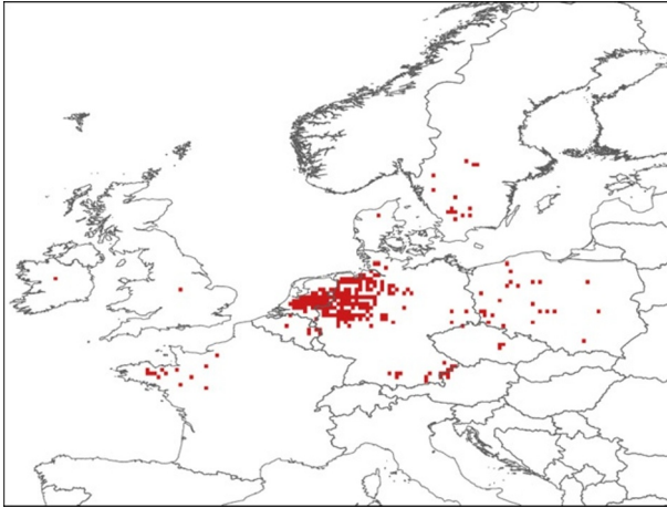
Figure 2.A2 In temperate grasslands, N is typically seen as limiting element. Assuming the direct effect of atmospheric N deposition on soil C:N (as in Box 2.4 ) and seen that soil C:N ratio co-determines the success of the plant and animal species occurring in natural grasslands and agroecosystems, it seems to us valuable to detect rural areas where the empirical soil C:N ratio is much lower than expected from the negative correlation between atmospheric N and soil C:N.
